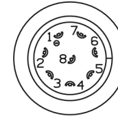
8 PIN FEMALE FUJISEIMITSU CONNECTOR
