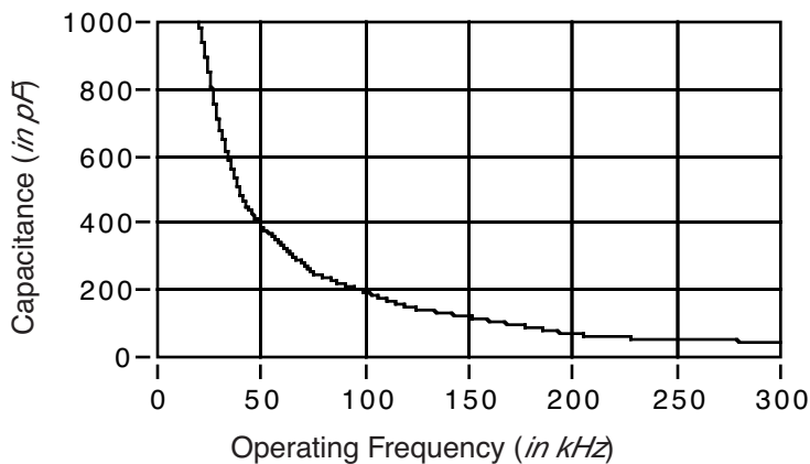
Figure 2. Capacitance vs. operating frequency
