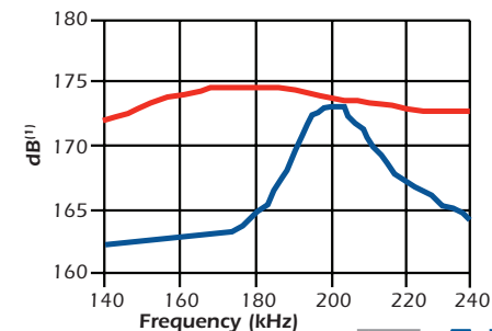
This Broadband transducer has a flat response and can run across the entire frequency range.
