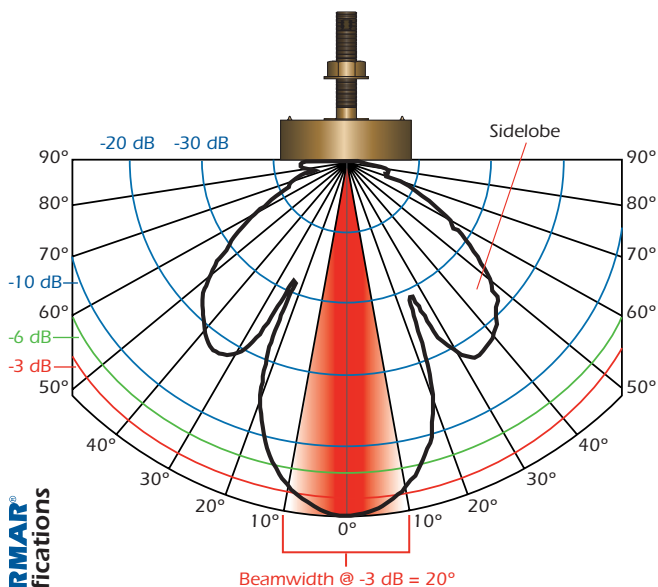
Beamwidth @ -3 dB = 20°
