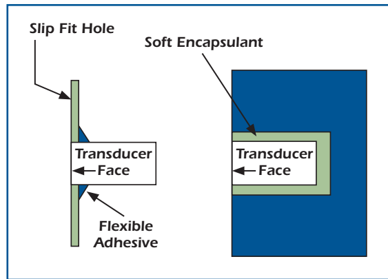
Figure 7: AT mounting examples
