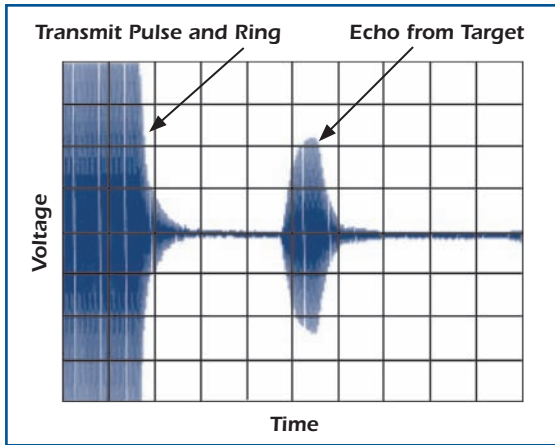
Figure 5: Transmit ring example
